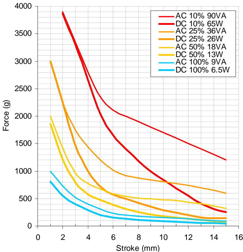
Force/Stroke Characteristics
