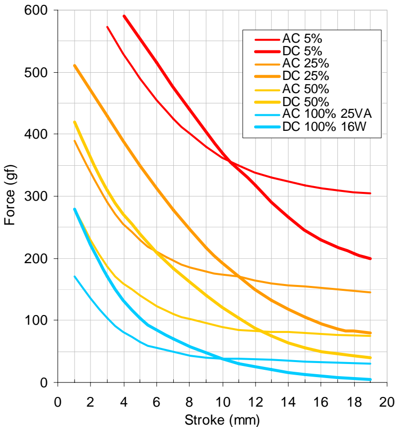
Force/Stroke Characteristics
