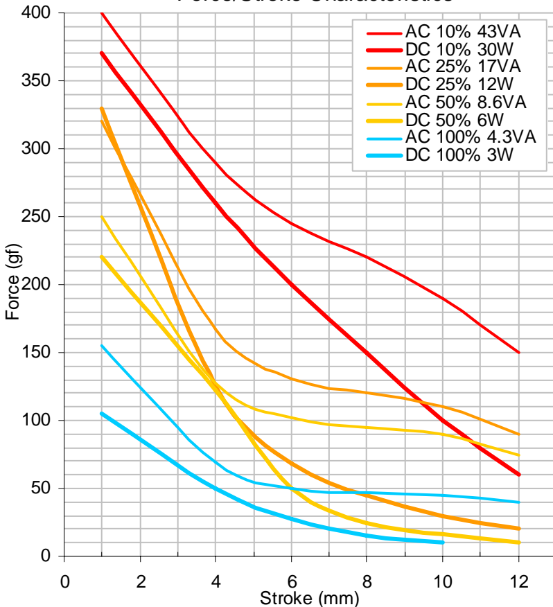
Force/Stroke Characteristics
